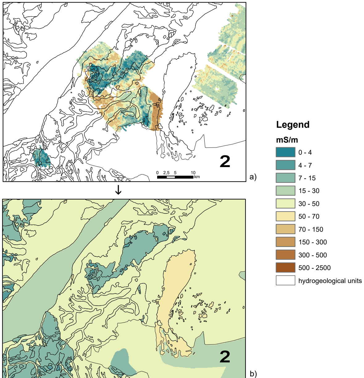
Figure 1 Example for extrapolation (b) of airborne electromagnetic data (conductivity) (a) to hydrogeological units in Eastern Austria (executed with ArcGIS).
