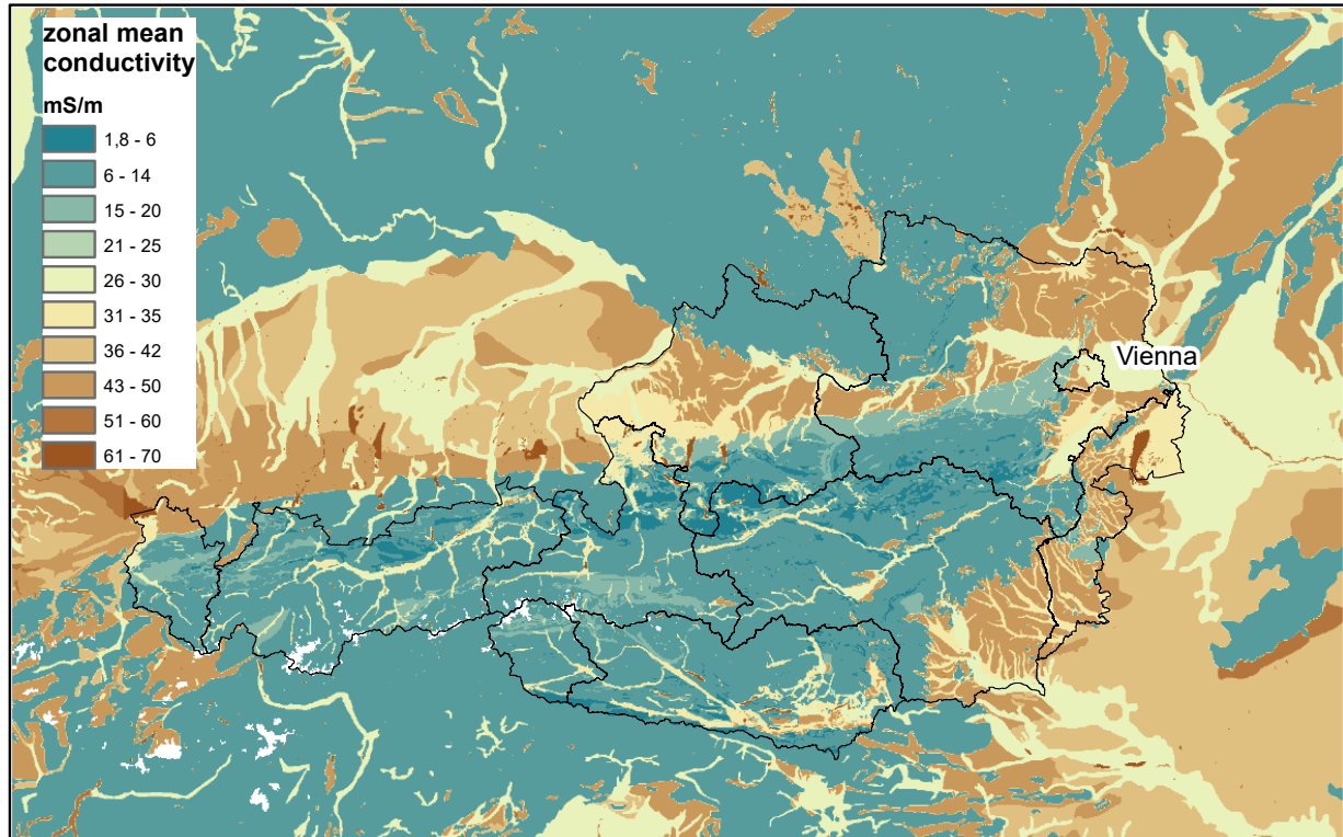
Figure 2 High-resolution subsurface conductivity model of Austria and its surroundings.
